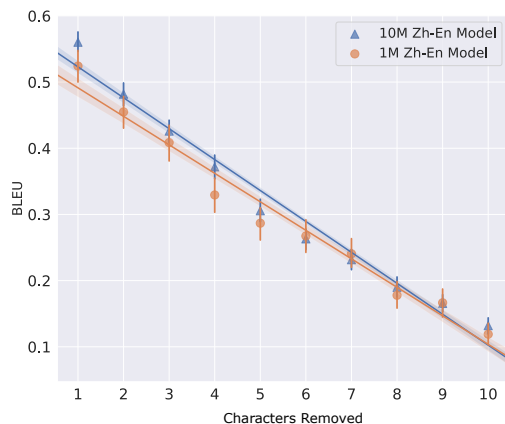
Figure 1: Zh-En BLEU as function of characters removed on valid sentences with 95% confidence intervals. There is a linear relationship, with average BLEU converging as more tokens are removed. The same is true on errors (not shown).
